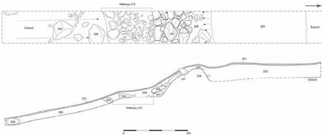
Figure 07: Trench 2, post-excavation plan and east-facing section
